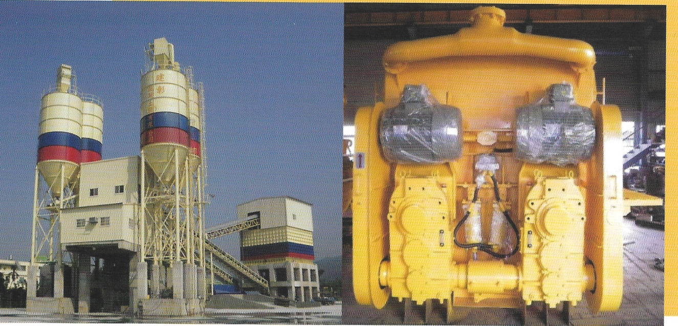
Wet Plant - 3m 3 Twin Shafts Mixer
